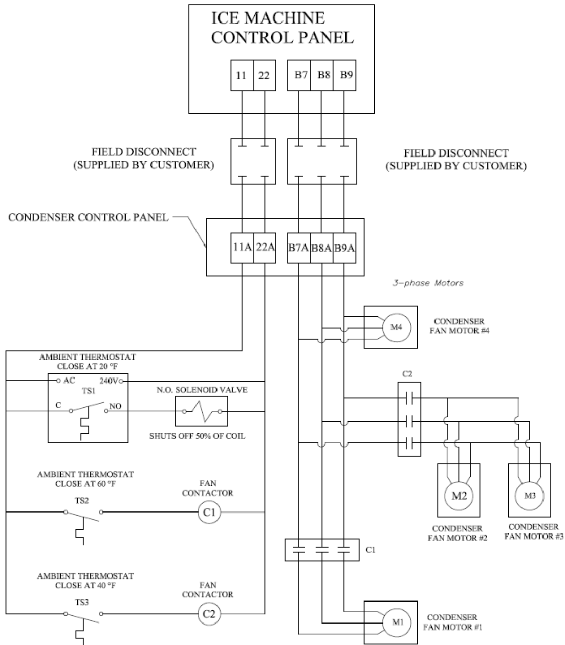
FIGURE – 18 Wiring For BOHN BNHS04A029 with Cold Weather Valve and Four Fans, 50/50 Condenser Split
