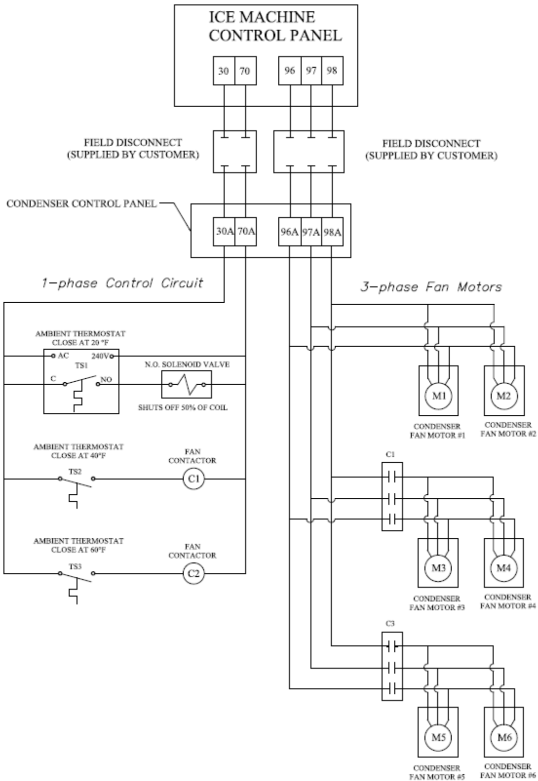
FIGURE – 18B Wiring For BOHN BNHD06A044 (Standard HFO10) Six Fan, 50/50 Condenser Split
