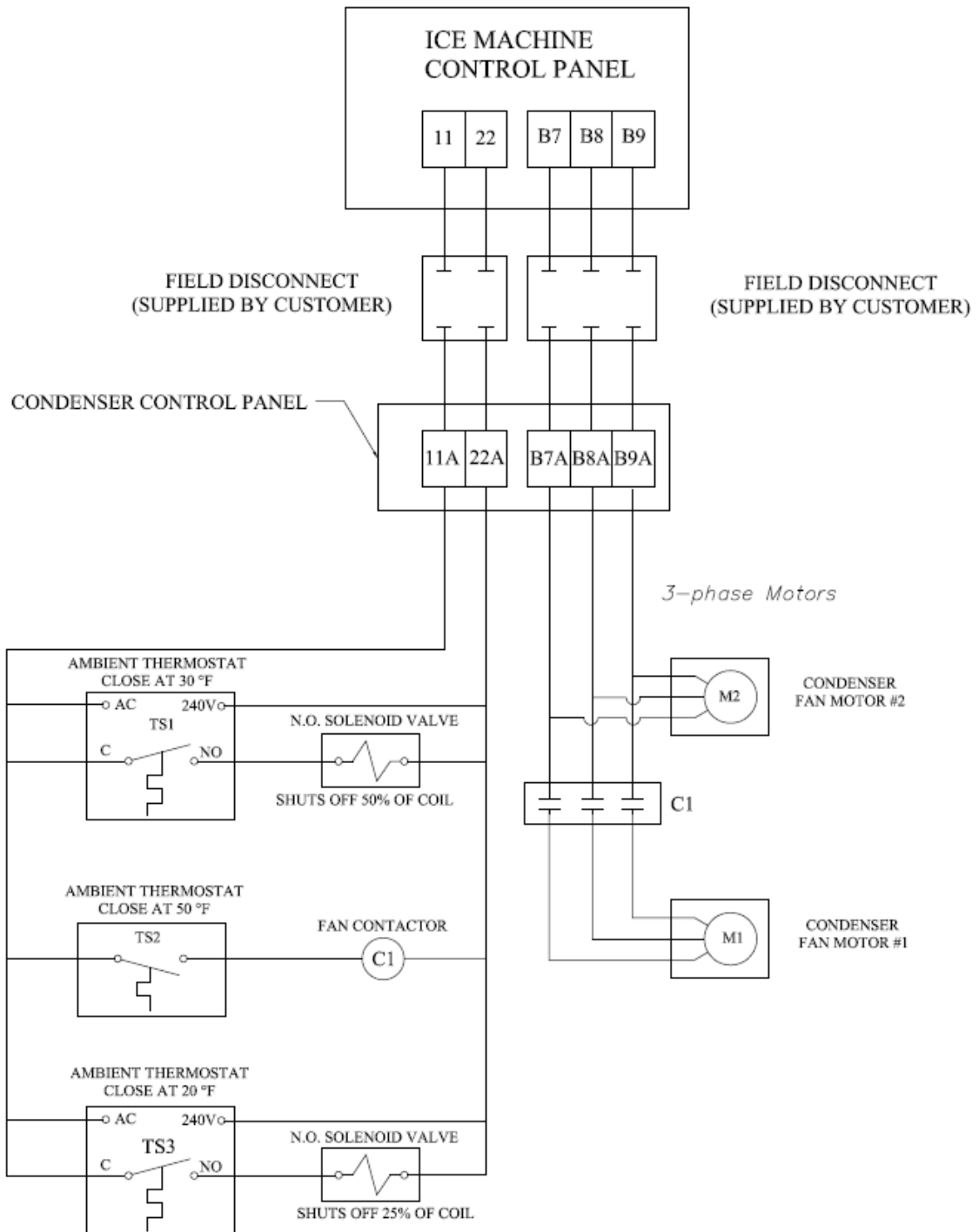
FIGURE – 17 Wiring For BOHN BNHS02A015(8)/BNHS02A015(12) with Cold Weather Valve and Two Fans, 50/25/25 Condenser Split
