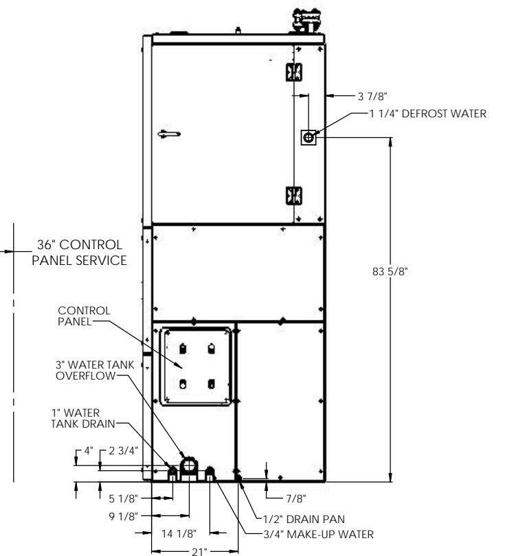
REAR ELEVATION SINGLE MODULE - TYP
