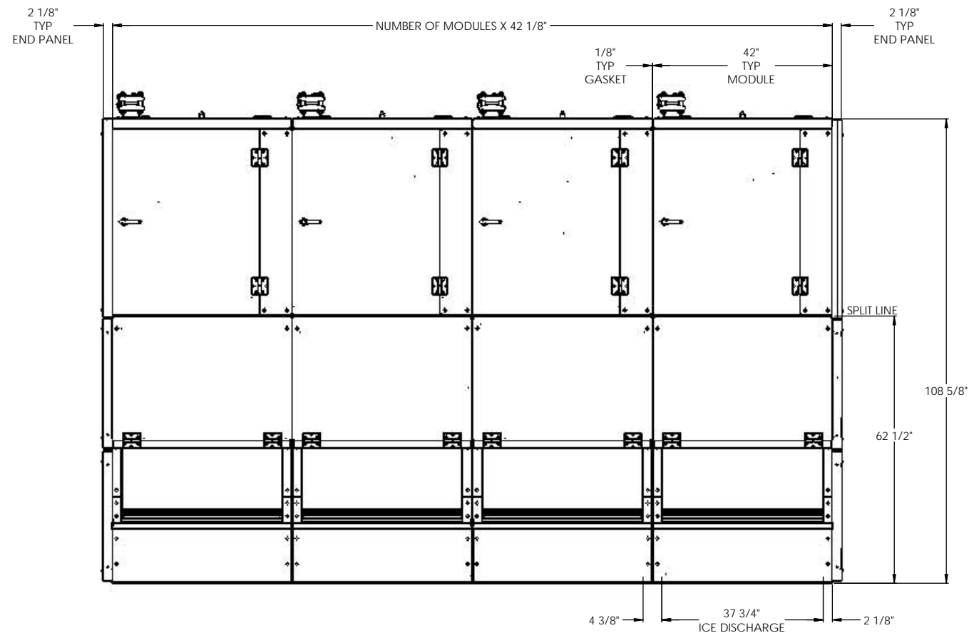
FRONT ELEVATION
