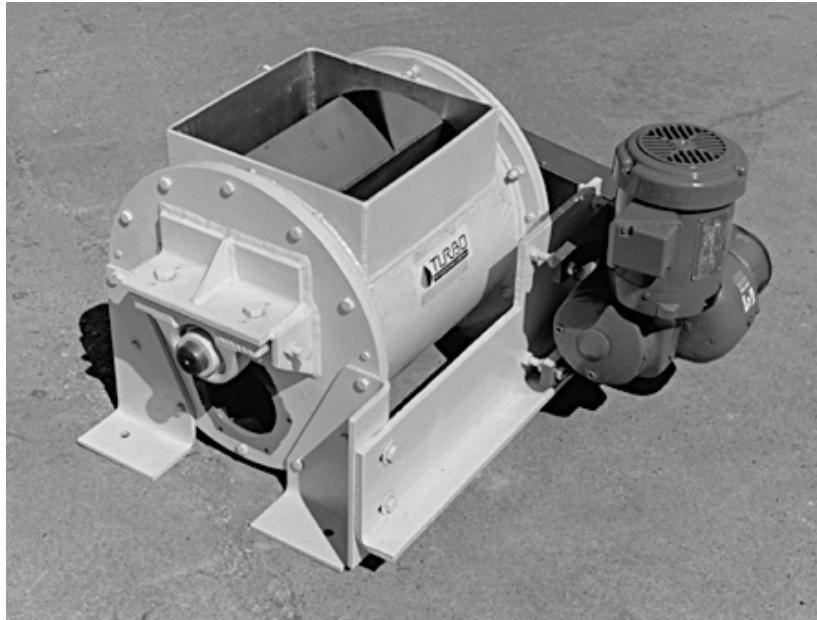
Rotary Valve
