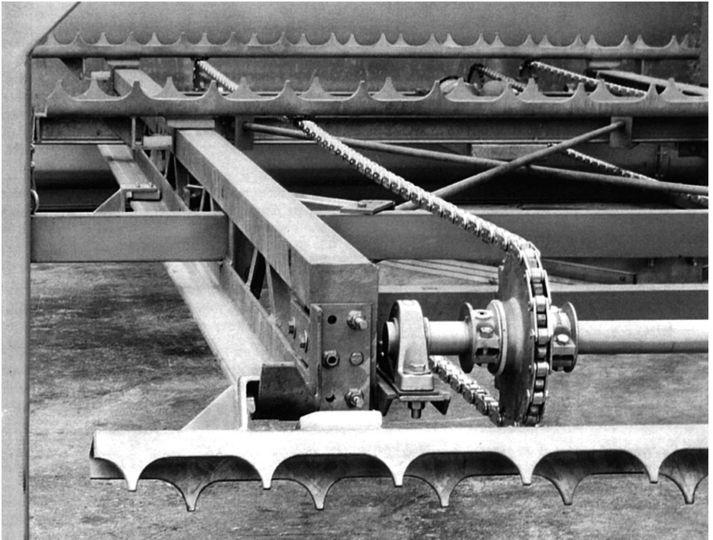
Automatic Rake Assembly without Optional Bin Structure and 180° Return Bends
